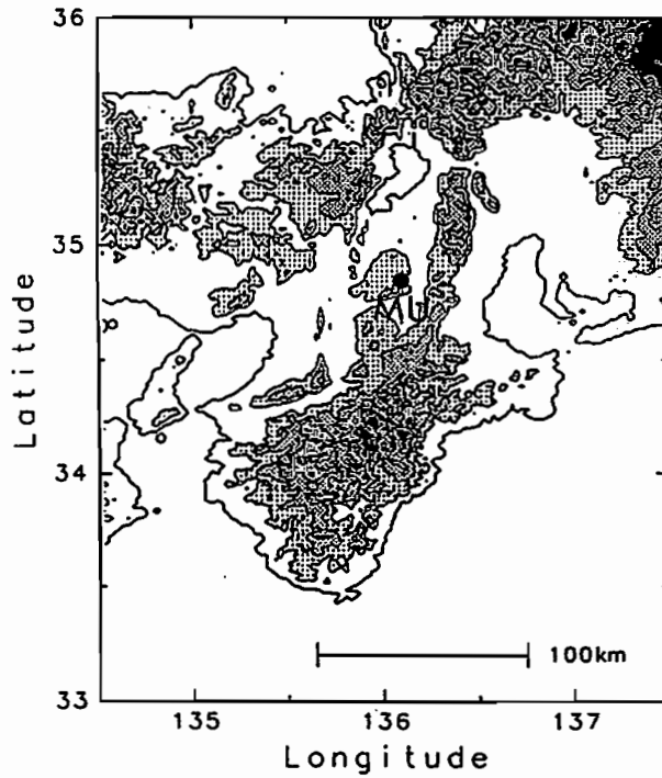
FIG. 12. A map of topography around the MU radar site. Contour interval is 250 m.
