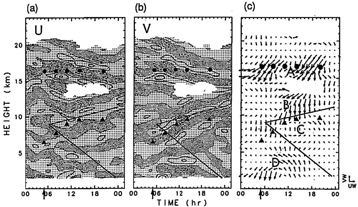
FIG. 15. Time-height sections of (a) zonal and (b) meridional wind components of disturbances with a vertical wavelength of 3 km in AT. Contour interval is 2 \text{ m s}^{-1} . Light and dark hatches show positive and negative wind velocities, respectively. Vertical momentum flux vectors associated with the disturbances are also presented (c), for which a smoothing was made by a low-pass filter with a cutoff length of 10 h instead of the average so as to see temporal and vertical variation of the vertical momentum flux. Rightward and upward unit vectors show eastward and northward vertical momentum fluxes of 0.1 \text{ m}^2 \text{ s}^{-2} , respectively. A thick arrow on the horizontal axis indicates the time when the typhoon passed near the MU radar site. Circles and triangles denote the tropopause and inversion layer, respectively.
