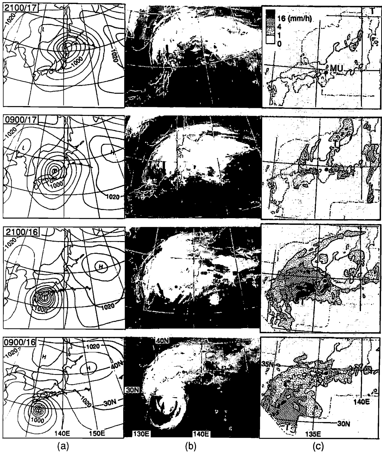
FIG. 2. (a) Synoptic charts of sea-level pressure in hectopascal, (b) IR pictures of GMS, and (c) the Radar-AMeDAS composite charts presenting precipitation per hour. Numerals in the top left of each figure in (a) denote local time and date. The typhoon center is indicated by "T" in (a) and (c), and by thick arrows in (b). Circles show the location of the MU radar. Dash-dotted lines in (c) show the boundaries in which the precipitation data exist.
