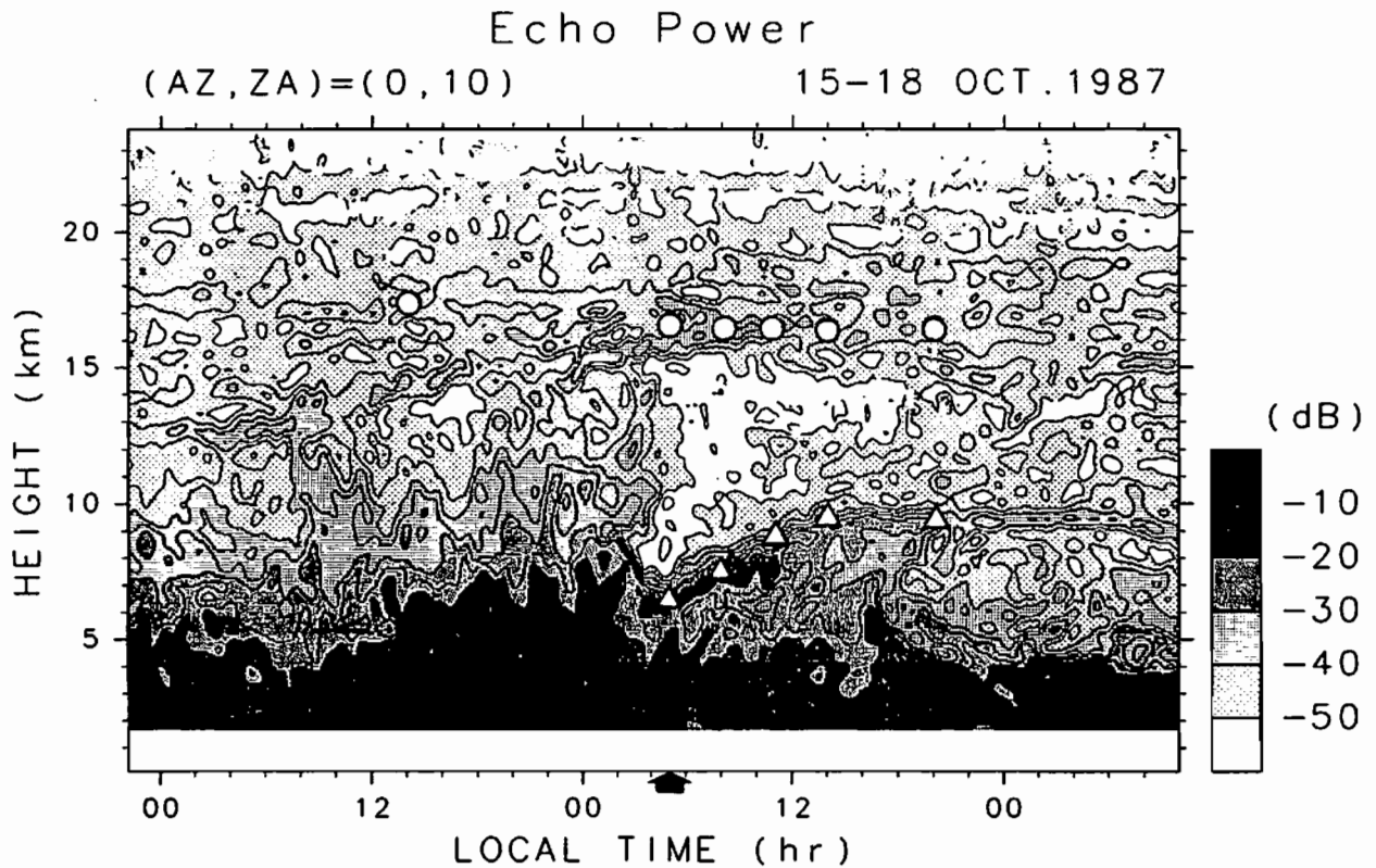
FIG. 4. A time-height section of echo power observed by a beam tilted to the north with a zenith angle of 10^\circ . Contour interval is 5 dB. A thick arrow on the horizontal axis denotes the time when the typhoon passed near the MU radar site.
