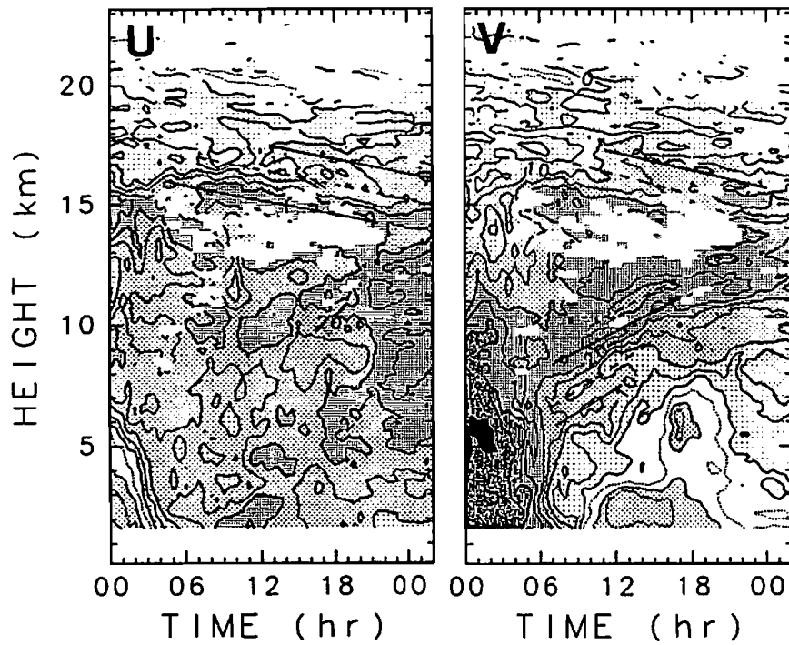
FIG. 14. Time-height sections of original (a) zonal and (b) meridional winds in AT.
