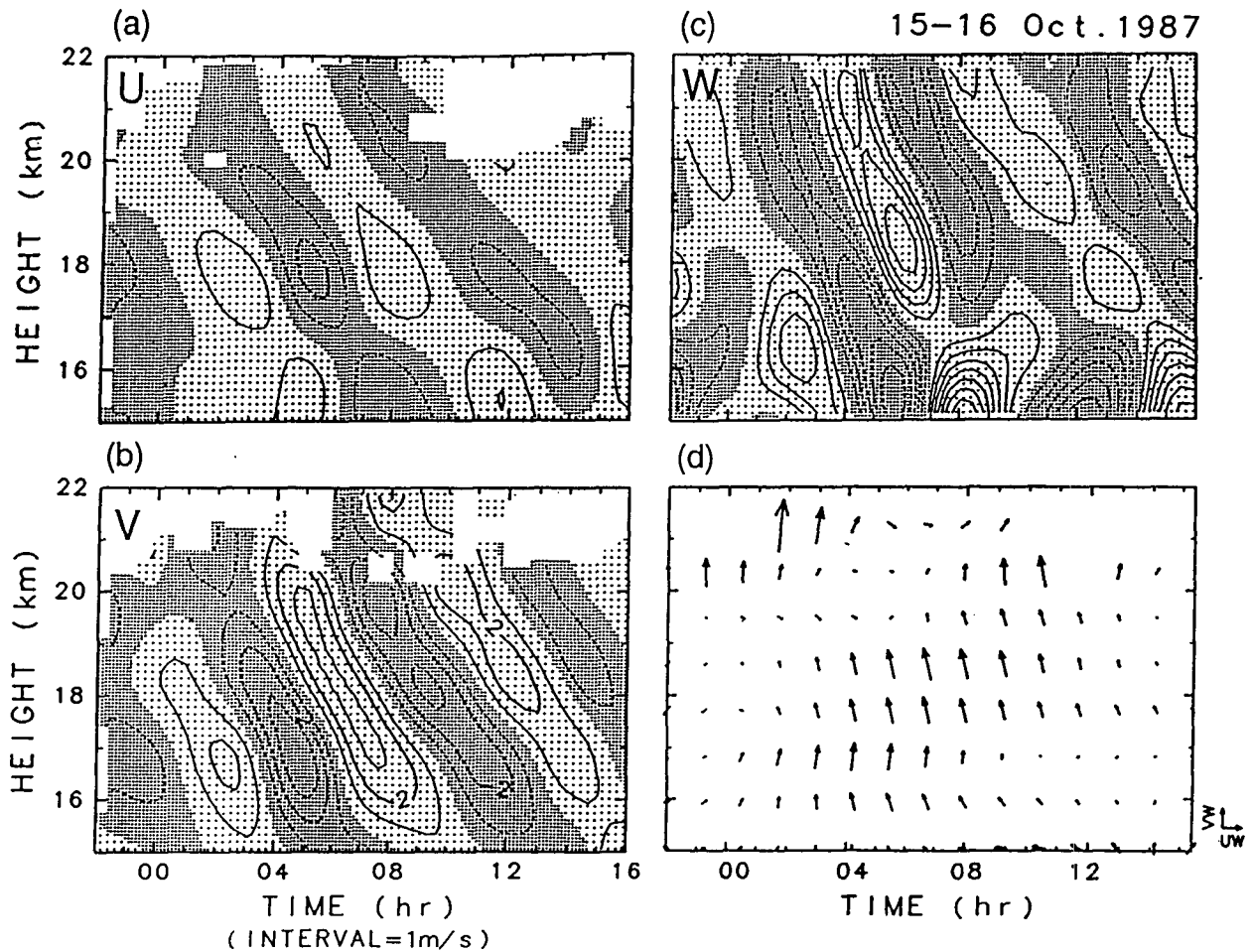
FIG. 18. A time-height section of (a) zonal, (b) meridional, and (c) vertical wind velocities and (d) vertical momentum flux vectors for an inertio-gravity wave observed about one day before the typhoon passage. Contour intervals are 1, 1, and 0.01 \text{ m s}^{-1} for (a), (b), and (c), respectively. A smoothing was made for the vertical momentum flux by a low-pass filter with a cutoff length of 10 h. Rightward and upward unit vectors in (d) show eastward and northward vertical momentum fluxes of 0.05 \text{ m}^2 \text{ s}^{-2} .
