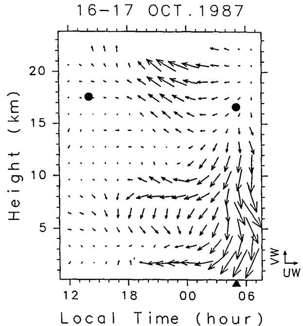
FIG. 10. A time-height section of vertical momentum flux vectors associated with fluctuations having periods less than 1 h in BT. Rightward and upward unit vectors show eastward and northward vertical momentum fluxes of 0.2 \text{ m}^2 \text{ s}^{-2} , respectively. A thick arrow on the horizontal axis indicates the time when the typhoon passed near the MU radar site. Circles denote the tropopause.
