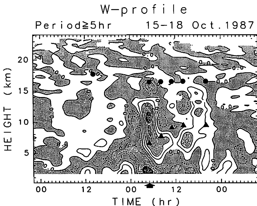
FIG. 11. Vertical wind components with periods longer than 5 h. Solid and dashed lines show positive and negative velocities, respectively. Contour interval is 0.25 \text{ m s}^{-1} . A thick arrow on the horizontal axis indicates the time when the typhoon passed near the MU radar site. Circles and triangles denote the tropopause and inversion layer, respectively.
