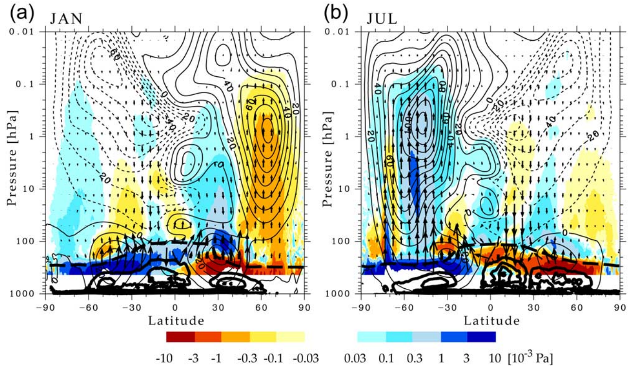
Figure 10. Zonal mean vertical flux of meridional momentum ( \rho_0 \overline{v'w'} ) associated with n \geq 43 waves (color) and zonal mean zonal wind (contours) in (a) January and (b) July. Arrows denote corresponding E-P flux as shown in Figures 8d and 9d. Bold dashed line denotes the tropopause, and solid contour lines denote monthly average values of zonal mean condensational heating rate in the troposphere (cumulus + large-scale condensation, contour interval of 1 \text{ K d}^{-1} ).
